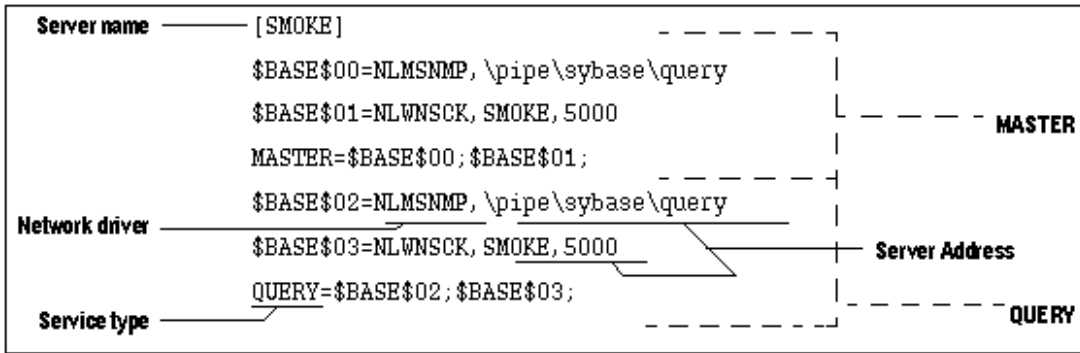
Figure 4-2: Components of the sql.ini file
